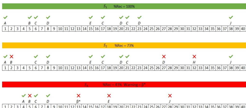
Figure 5. Evaluation of the V-net with the event sequences S_1 , S_2 , and S_3
