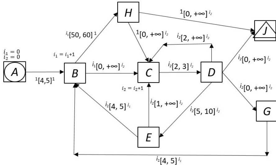
Figure 3. Solution using V-net
