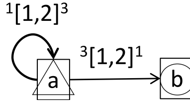
Figure 2. Example of a V-net ( V_N )
