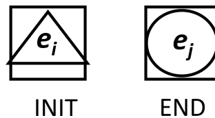
Figure 1. Graphical representation of INIT and END
