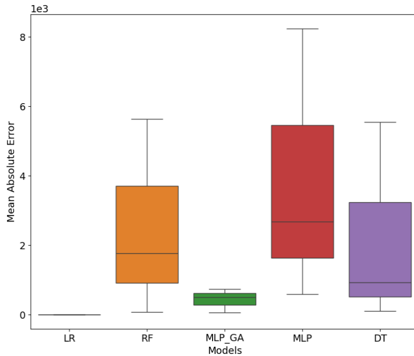
Figure 16. Comparison of prediction errors MAE for Institution III using artificial intelligence models
