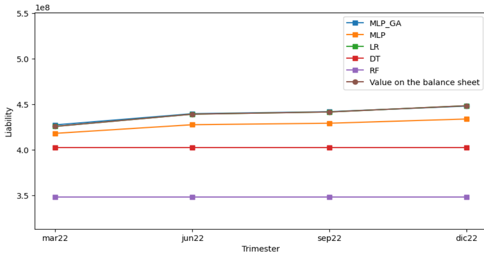
Figure 6. Comparison of actual values from the test set and predicted values for the Liabilities account using artificial intelligence models with default hyperparameters –quarterly analysis– for Institution I.
