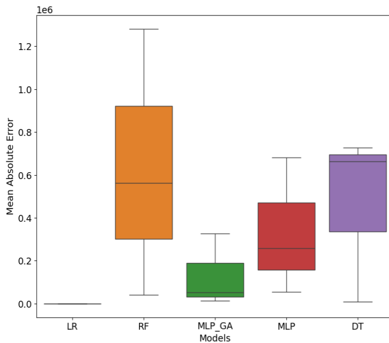
Figure 17. Comparison of prediction errors MAE for Institution IV using artificial intelligence models
