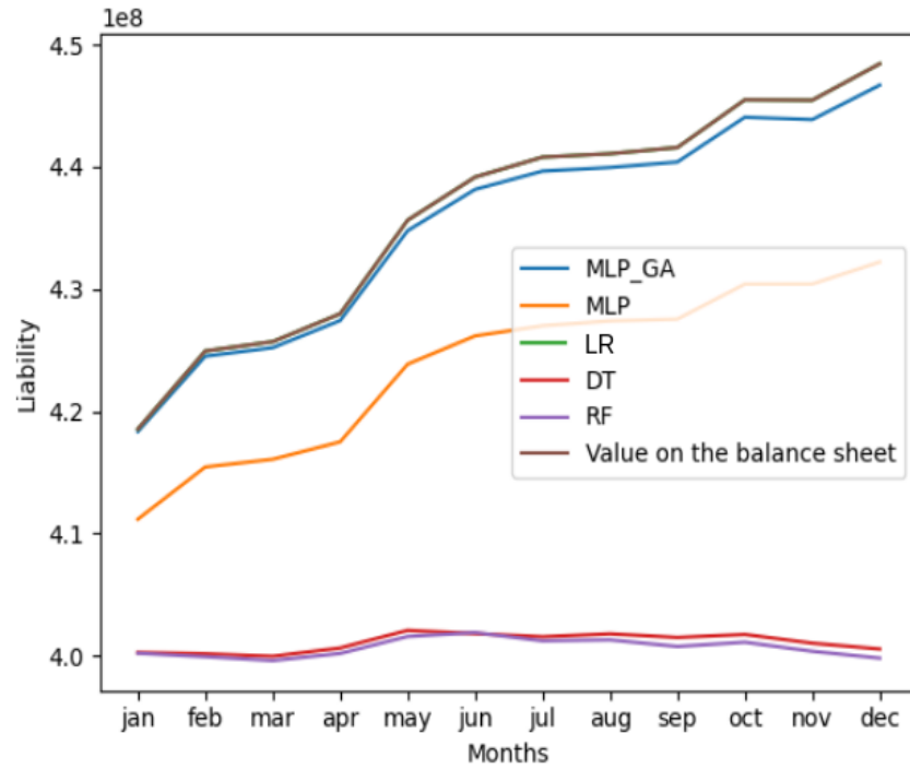
Figure 4. Comparison between the actual values from the test set and the predicted values for the Liabilities account obtained using artificial intelligence models with default hyperparameter settings for Institution I
