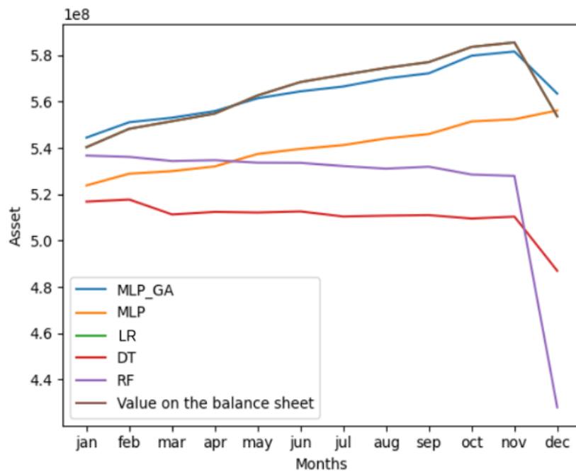
Figure 3. Comparison between the actual values from the test set and the predicted values for the Assets account obtained using artificial intelligence models with default hyperparameter settings for Institution I
