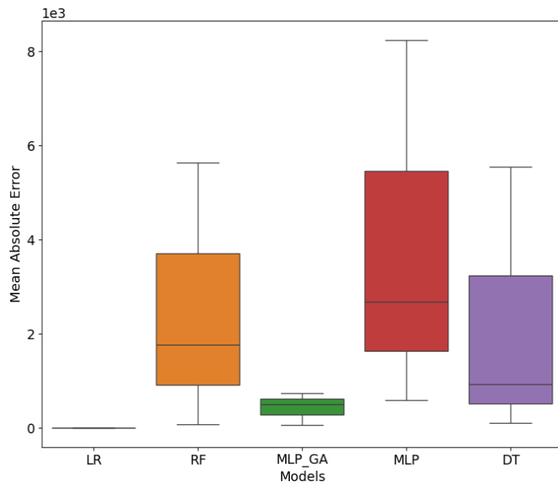
Figure 15. Comparison of prediction errors MAE for Institution II using artificial intelligence models
