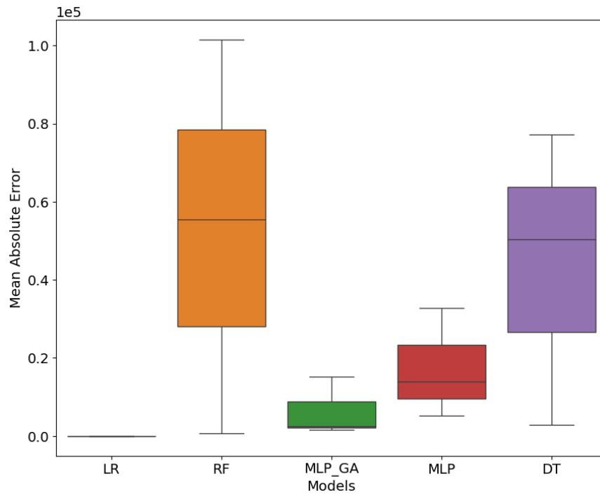
Figure 14. Comparison of prediction errors MAE for Institution I using artificial intelligence models
