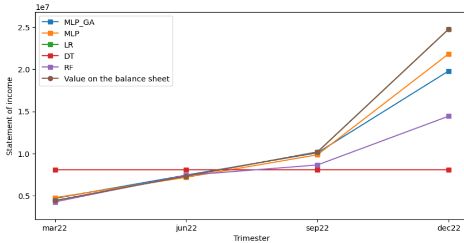
Figure 8. Comparison of actual values from the test set and predicted values of the profit or loss account from the income statement using artificial intelligence models –quarterly analysis– for Institution I
