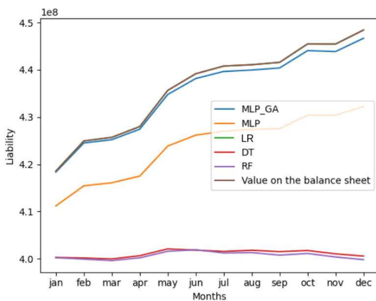
Figure 4. Comparison between the actual values from the test set and the predicted values for the Liabilities account obtained using artificial intelligence models with default hyperparameter settings for Institution I
